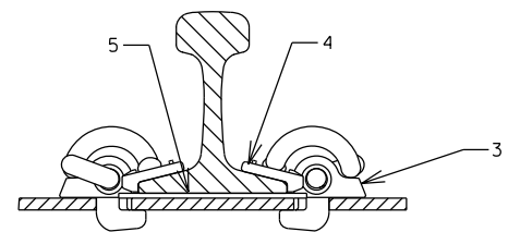
Typical Insulated Rail Assembly
