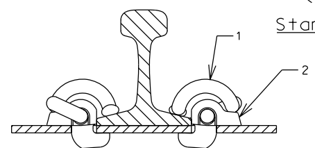
Typical Uninsulated Rail Assembly
